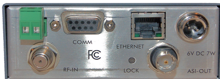
DTV-R3000: Rear Panel
